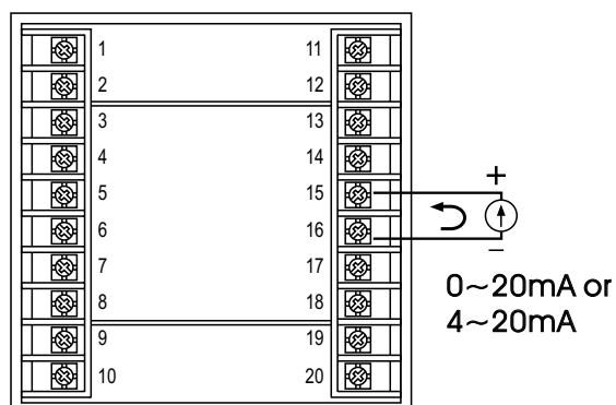
Figure 2.10 Input 2 Linear Current Wiring
