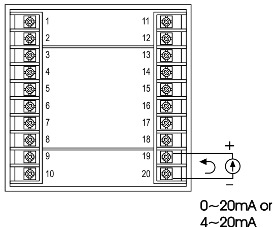
Figure 2.8 Input 1 Linear Current Wiring
