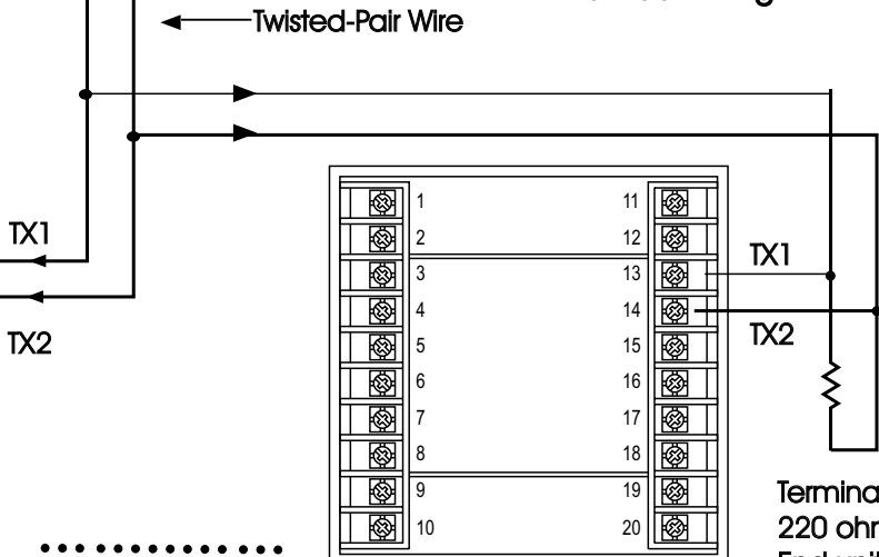
Figure 2.17 RS-485 Wiring
